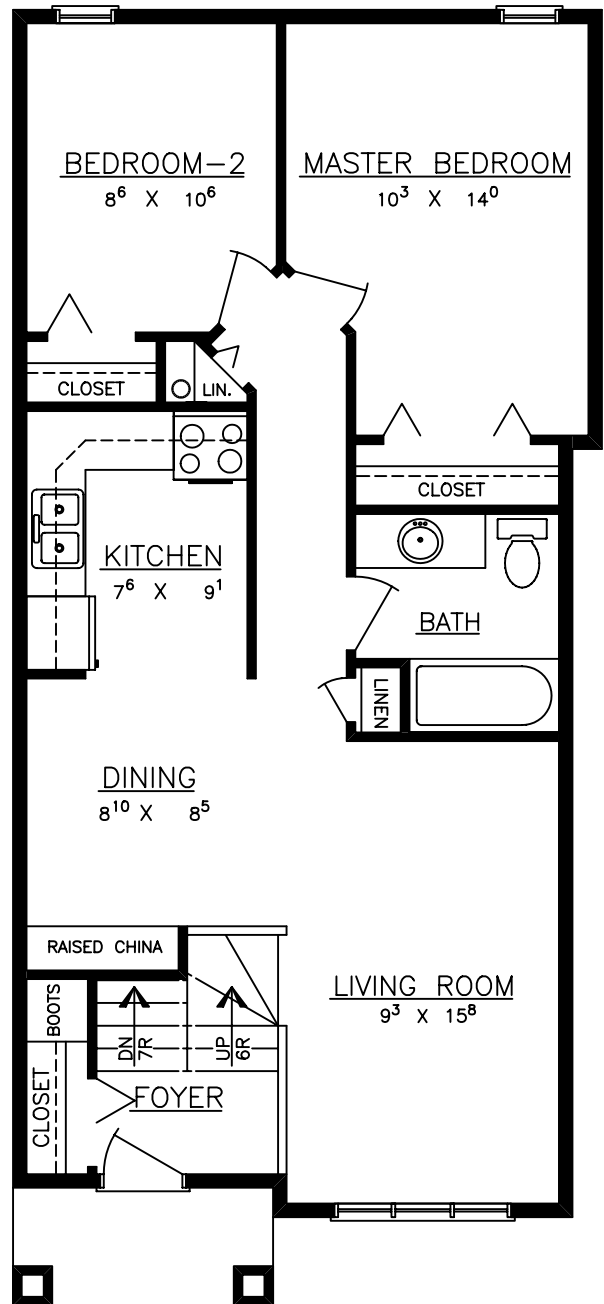
FLOOR PLAN
